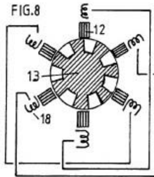
Fig. 8 shows a six stator pole configuration with a seven pole rotor and depicts a schematic series connected linking of the magnetizing windings of diametrically opposite stator poles.
