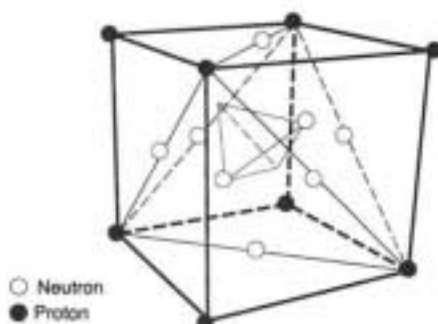
Figure 16 PROBABLE LOCATION OF THE OXYGEN-16 NEUTRONS AND PROTONS
