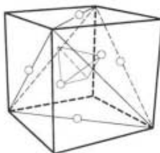
Figure 15 PROBABLE LOCATION OF CARBON NEUTRONS
