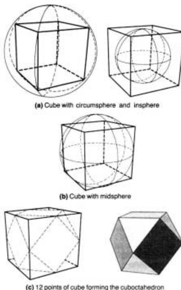
Figure 3 FORMING THE CUBOCTAHEDRON FROM THE CUBE The cube is shown (a) with the circumsphere, which is internally tangent to the 8 vertices, and insphere, which is tangent to the interior of the 6 faces. The midsphere (b) is tangent to the midpoints of the 12 edges. When these 12 points are connected (c), the figure formed is the Archimedean solid known as the cuboctahedron. The midsphere of the cube is the circumsphere of the cuboctahedron.
