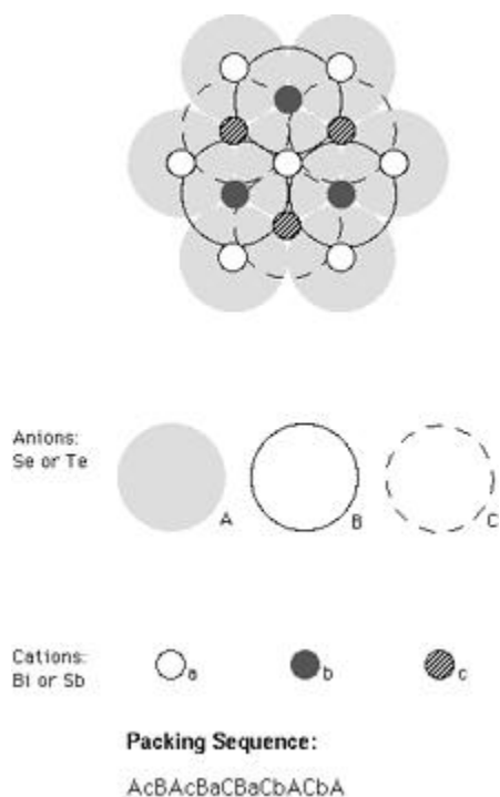
Figure 8. Top view (looking down the crystal's c-axis) of the bismuth telluride unit cell. Large circles represent anions, small circles represent cations. Letters denote the different relative arrangements of atomic planes; an upper-case letter indicates a close-packed plane of anions; a lower-case letter indicates a plane of cations in octahedral holes midway between anion planes.
