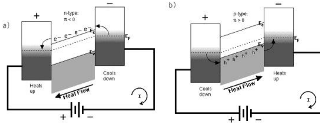
Figure 5. Illustration of the Peltier effect for a semiconductor between two pieces of metal. (a) n-Type semiconductor. Electrons flow from right to left in the semiconductor, carrying heat from the right to the left side of the semiconductor, opposite to the electric current direction; \Pi is negative. (b) p-Type semiconductor. Holes flow from left to right in the semiconductor, carrying heat from the left to the right side of the semiconductor, in the same direction as the electric current; \Pi is positive. E_C , E_V , and E_F refer to the energies of the conduction band edge, the valence band edge, and the Fermi energy (or electrochemical potential), respectively. Figure adapted from Hannay, N. B. Semiconductors ; Reinhold: New York, 1959; p 41.
