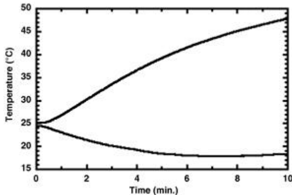
Figure 2. Temperature at the two heat sinks of the thermoelectric module as a function of time. The module was turned on at time zero with a polarity corresponding to cooling the food chamber. A similar temperature profile was obtained when the polarity was reversed, corresponding to heating the food chamber.
