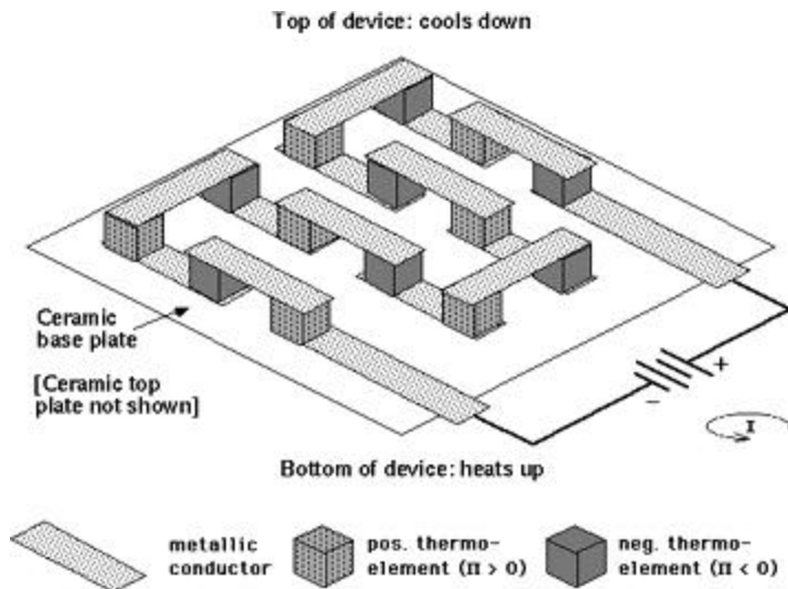
Figure 10. Thermoelectric cooling module. An array of positive and negative thermoelements are arranged between two ceramic plates so that they are electrically in series but thermally in parallel. All of the elements move heat from the top to the bottom of the module. Note that all of the metallic conductors are entirely in the plane of the top plate or the bottom plate.
