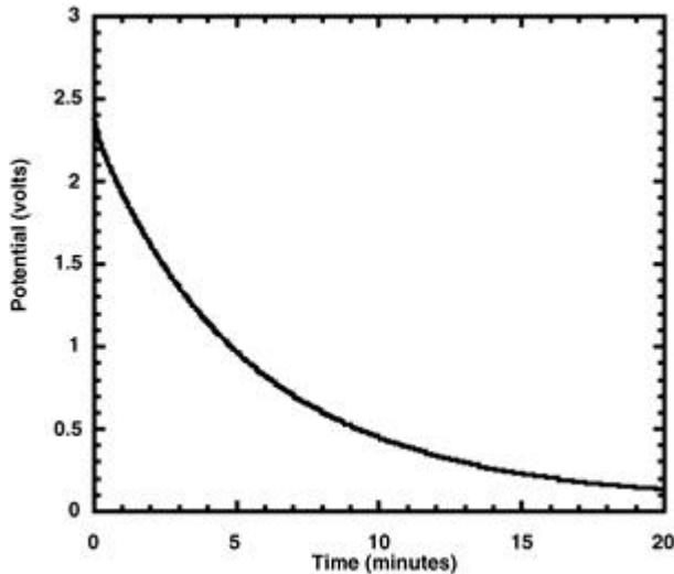
Figure 3. Voltage produced by the thermoelectric module after the temperature gradient shown in Fig. 2 was established ( t=0 in this figure corresponds to t=10 in Fig. 2). A similar profile was obtained if the module was powered with the polarity reversed.
